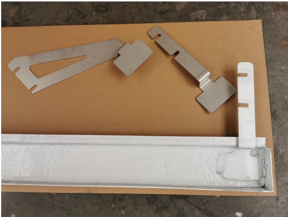
Glue the bracket into the sideskirt. The bracket mounts on the original sideskirt mounting points.
